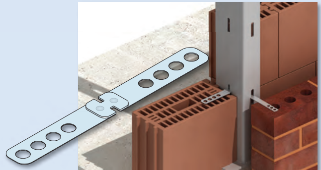
Ancon CCB-SNS Tie Two way windpost tie
