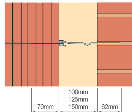
CCB3 and CCB4 Wall Ties
