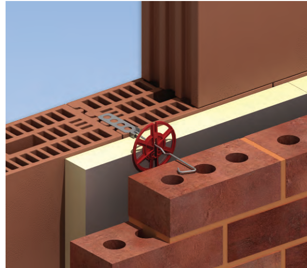
CCB3 and CCB4 Wall Ties
