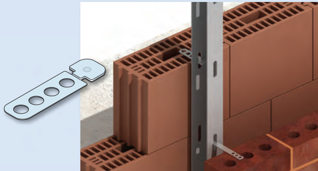
Ancon CCB-SPN Tie One way windpost tie
